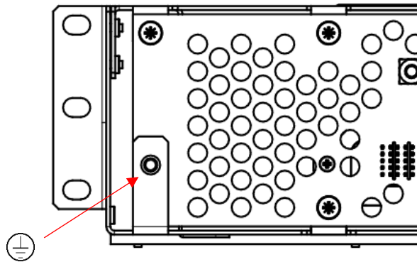
Figure 10: Chassis Earth Point
