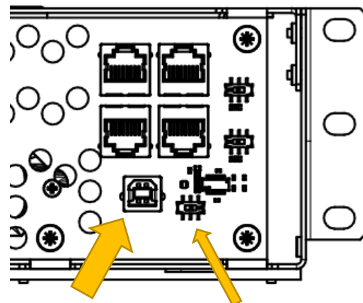
Figure 3: USB-B Programming Port and Toggle Switch
